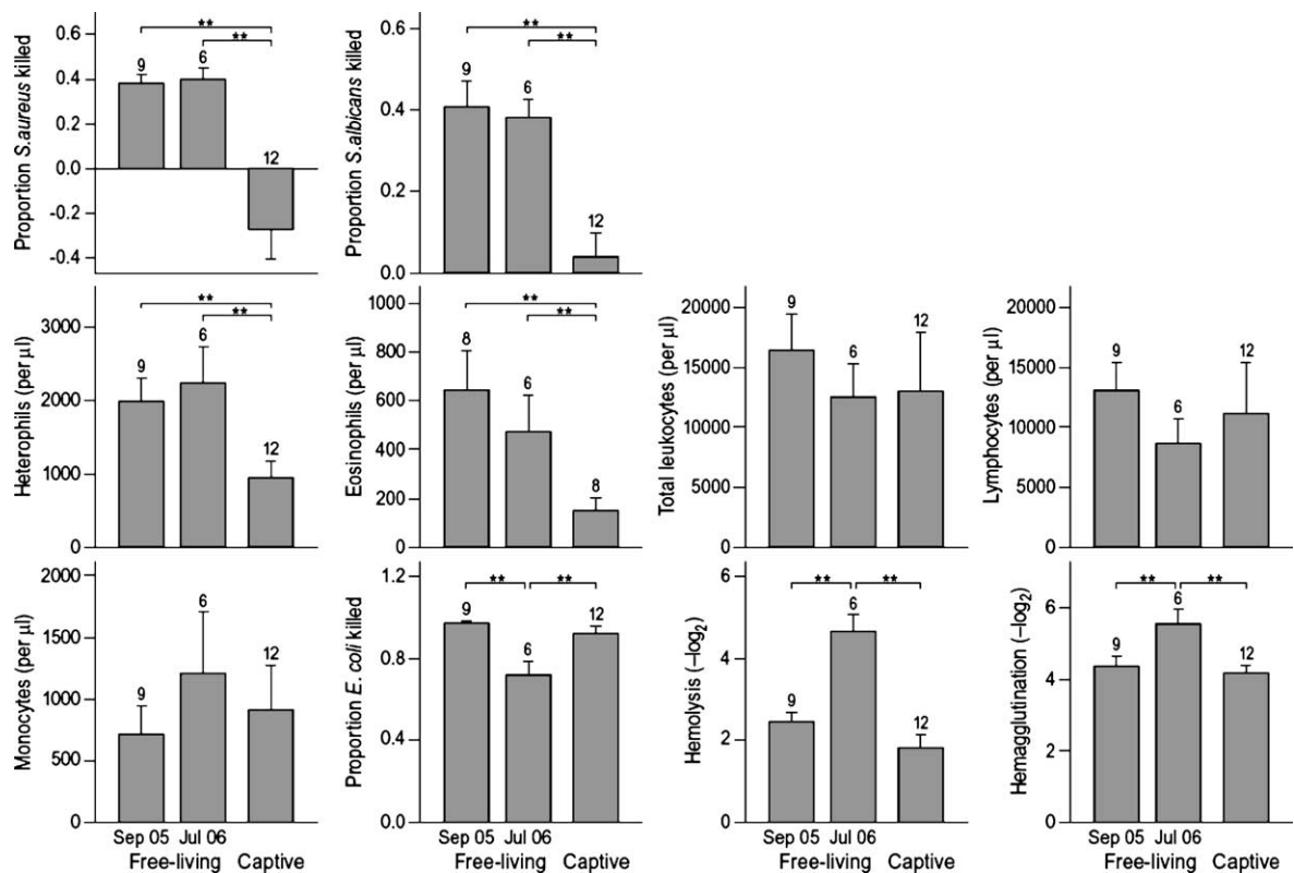
Figure 1. Immune function in captive versus free-living red knots. For E. coli killing and leukocyte concentrations statistics were performed on transformed values, but raw data are shown here for ease of interpretation. Bars indicate mean \pm SE and sample sizes are indicated above the bars (lower for eosinophil count because zero values are not included). Significance from post-hoc Tukey tests is presented here as P < 0.05 (*) and P < 0.01 (**).
