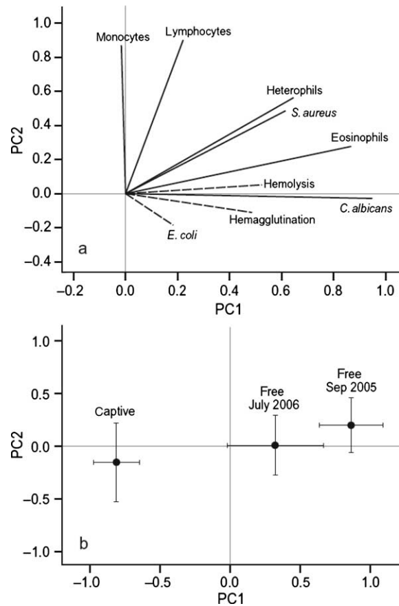
Figure 2. (a) Relationships between immune measures. The axes represent the first two components of a principal component analysis. Vectors are the loadings of each immune measure and the length of the vector indicates the strength of the relationship (the R^2 value) or how much of the variation in an immune measure is explained by the two axes. Dashed vectors are measures best explained by PC3 (see Table 1 for component loadings). The angle between two vectors gives the degree of correlation between them. Adjacent vectors are highly correlated with each other, orthogonal ( 90^\circ ) vectors are uncorrelated, and vectors pointing in opposite directions ( 180^\circ ) are negatively correlated. (b) The groupings of principal component scores (captive birds, free-living birds caught in September 2005 and free-living birds caught in July 2006). For each group the mean \pm SE of PC1 is plotted against the mean \pm SE of PC2. Captive and free-living birds are distinguished on PC1 but not on PC2.
