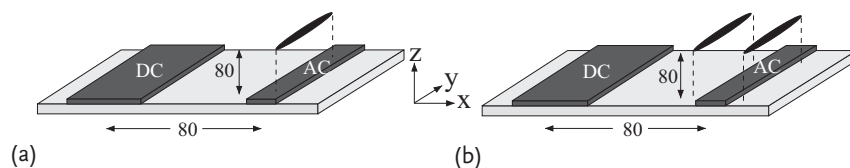
Figure 12.7 Atoms confined to single-well (a) and double-well (b) potentials induced by RF manipulation 80 \mu\text{m} above the chip surface.
