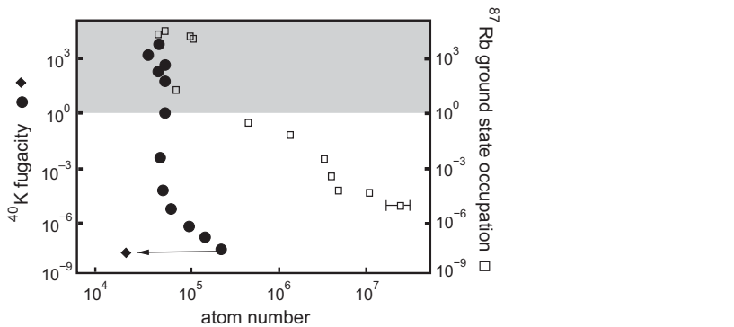
Figure 12.3 Sympathetic cooling to dual ^{40}\text{K} - ^{87}\text{Rb} quantum degeneracy. Spin-polarized fermions without a bosonic bath cannot be successfully evaporatively cooled (diamond). However, if bosonic ^{87}\text{Rb} (squares) is evaporatively cooled, the fermionic ^{40}\text{K} is sympathetically cooled (circles) by thermalizing elastic collisions with ^{87}\text{Rb} . The vertical axes
