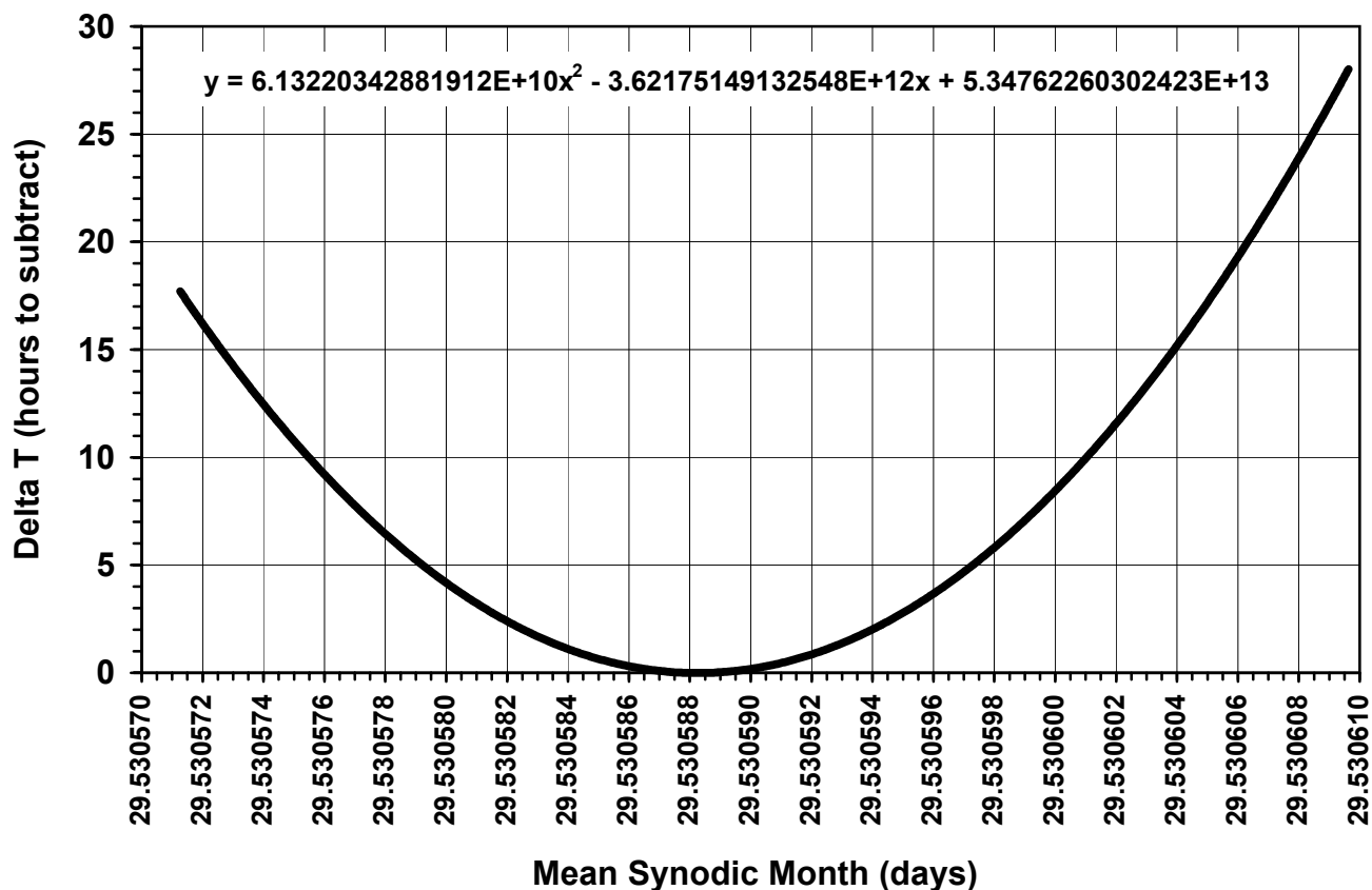
Delta T vs Mean Synodic Month
