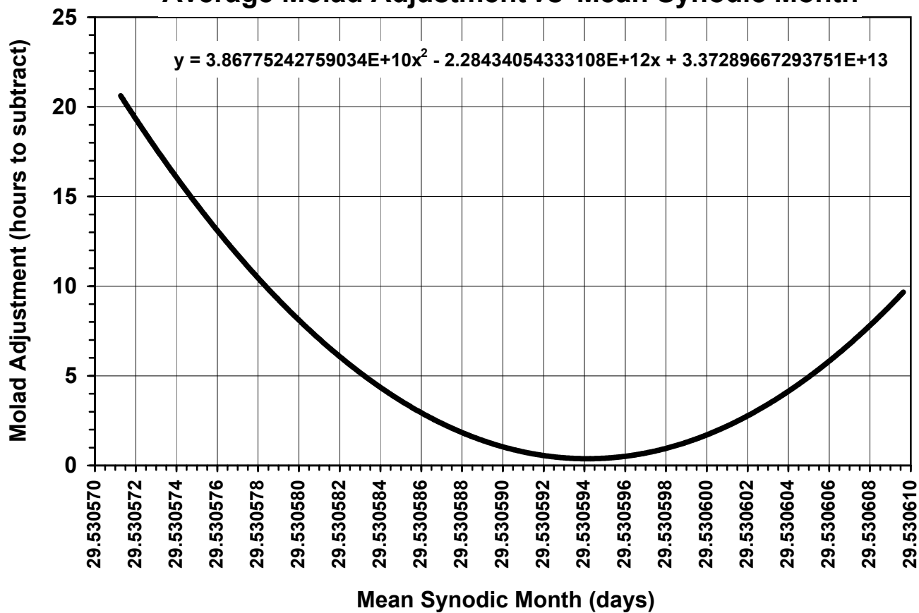
Average Molad Adjustment vs Mean Synodic Month
