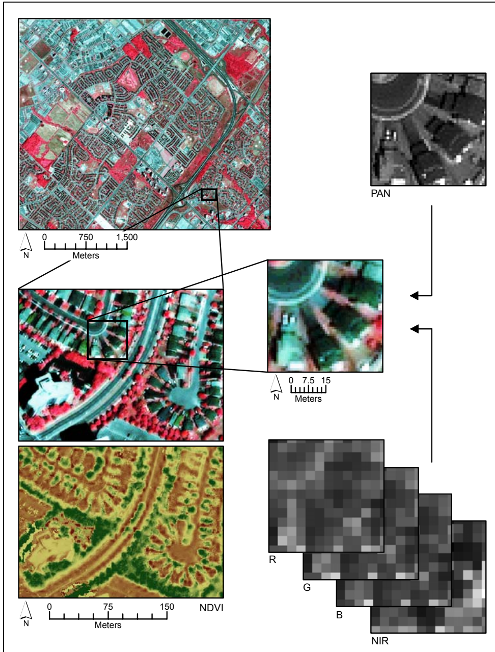
Figure 3.2: Ikonos imagery of the study area, including raw data and derivatives. The 4 spectral bands (lower right) were merged through PAN-sharpening with the PAN layer (upper right). An NDVI (lower left) was calculated to better distinguish vegetated and non-vegetated areas.
