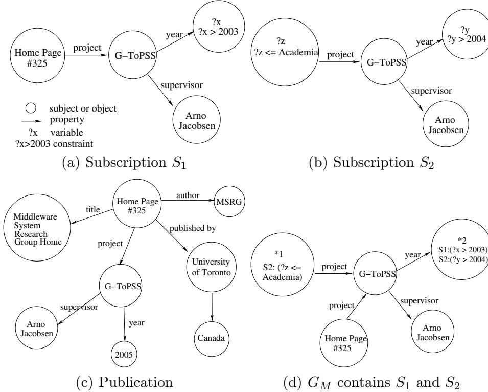
Fig. 5. Example subscriptions, publication and G_M
