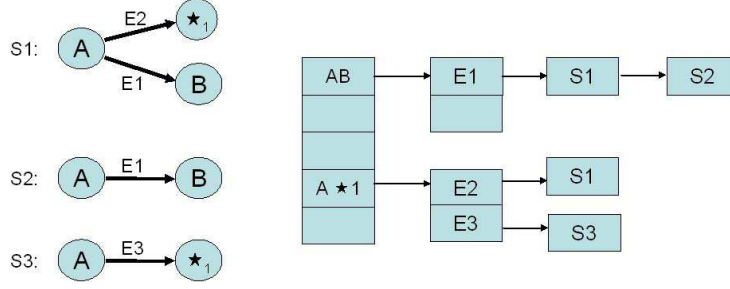
Fig. 7. Data Structure
