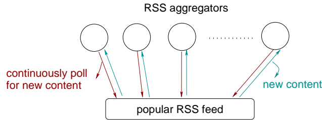
Fig. 1. Current RSS dissemination architecture
