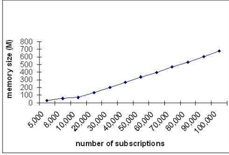
(a) Memory vs. #subscriptions
