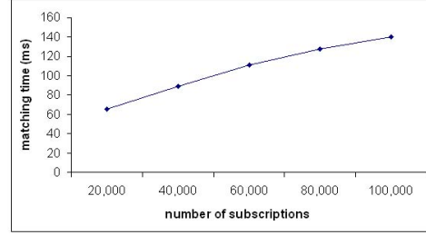
(b) Matching time vs. #subscriptions
