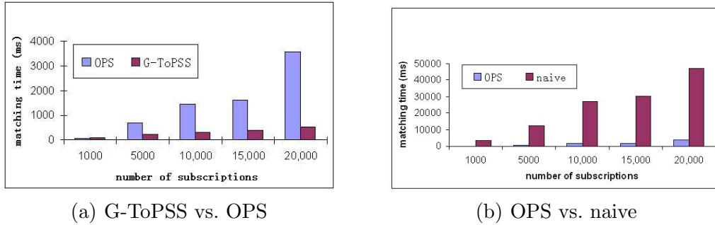
Fig. 10. Compare G-ToPSS with other algorithms
