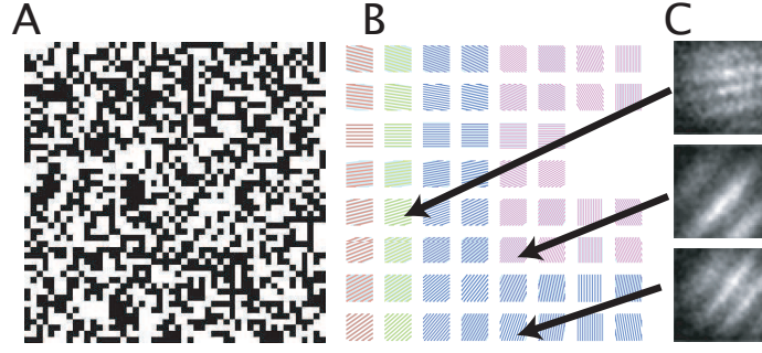
Figure 6. PFCA Calibration. Transfer functions of each pixel are found by presenting 6710 random binary 50 \times 50 calibration images (A) on a CRT screen (presentation time 16.7 ms each) to the array (B) and performing reverse correlation between the observed photocurrent of each sensor and the image presented. The kernels of three ASPs are shown (C); these resemble Fourier components.
