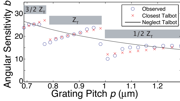
Figure 3. Closest Talbot Pattern Determines b . Observed b(p) agrees better with the assumption that z_{\text{effective}} equals the closest optimal Talbot depth, and not the manufactured depth. Blue circles: measured b as a function of pitch for incident green light on a series of devices spanning a range of p from 0.7 to 1.3 microns. Red xs: modeled b assuming Equations 2.1 and 2.3. Black line: modeled b assuming z_{\text{effective}} = z and Equation 2.1. Grey bars: depth of closest Talbot pattern.
