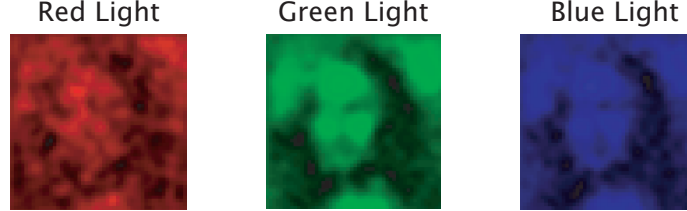
Figure 9. Three Colour Image Reconstructions. Using the basis functions \mathbf{H} obtained from red, green and blue calibration runs, the first prototype chip is able to resolve light images other than at the design wavelength (520nm). The center green image is identical to that of Figure 8B on the left.
