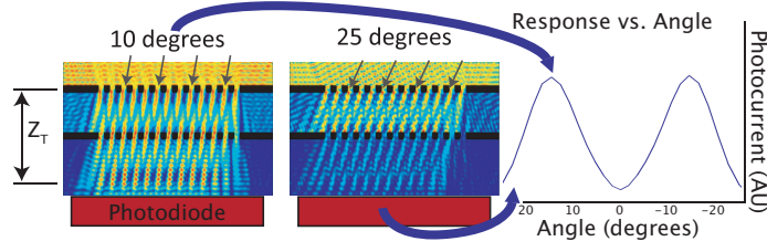
Figure 2. Interaction Between Incident Light and ASPs. Left: light incident at 10^\circ produces spatial maxima that align with gaps in the second grating, resulting in a large photocurrent. Center: light incident at 25^\circ produces spatial maxima that are largely blocked by the second grating, resulting in a small photocurrent. Right: photocurrent as a function of incident angle is a sinusoidal function.
