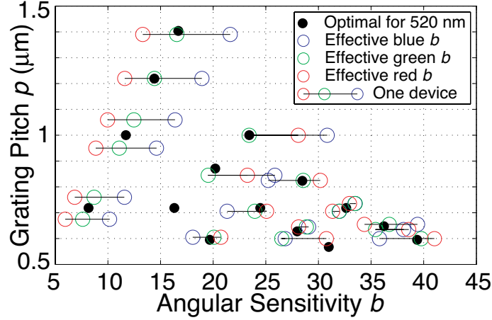
Figure 4. Selecting Devices for the PFCA. Filled black circles indicate manufacturable devices with maximal m for 520nm light; open circles indicate p and ( \lambda -dependent) b for the suite of devices we manufactured.
