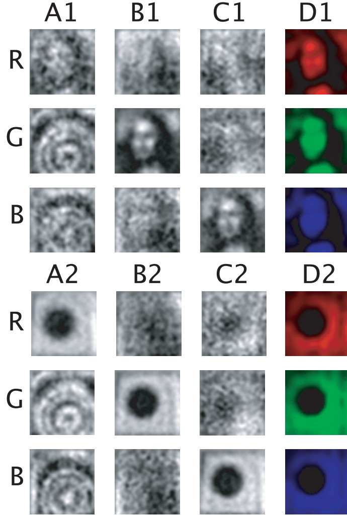
Figure 11. Blind Colour Imaging. We show reconstructions of test images 1 & 2 without foreknowledge of the colour of incident light. R, G and B rows: presented images were red, green and blue. A columns: image reconstructed using Equation 2.7 based on \mathbf{H} calibrated using red light. B & C columns: as for A, but using green- and blue-calibrated \mathbf{H} matrices. D columns: reconstruction based on Equation 5.1 without any assumption about colour, or that the image is monochromatic.
