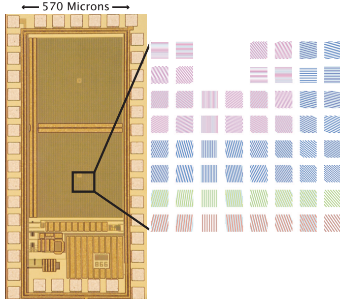
Figure 5. Manufactured PFCA. Concentric rings of ASPs with increasingly high b yield a complete Fourier description of the light intensity from the far field. Slowly varying orientation is evident from the enlarged section, where schematics show different metal layers in different colours.
