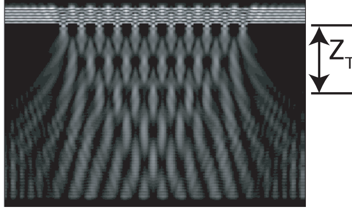
Figure 1. The Talbot Effect. Wave simulation of monochromatic light striking a grating at the normal. The grating periodicity is recapitulated at regularly-spaced depths below the grating; a phenomenon known as the Talbot effect. The Talbot depth Z_T is shown at right.
