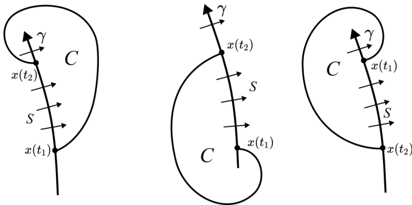
Figure 21: Other cases for showing monotonicity. Note in the second two cases it is the 'complement' of C that is positively invariant.
