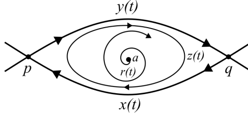
Figure 18: Example of limit sets, assume p, q, a are equilibria
