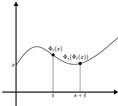
Figure 15: The semigroup property of flow. Evolving for time s from \Phi_t(x) corresponds exactly with evolving for time s + t from x .
