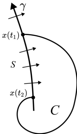
Figure 20: Solutions are trapped inside C after entering it
