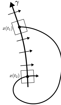
Figure 22: x(t_n) must eventually be in the top box but this breaks monotonicity on \gamma
