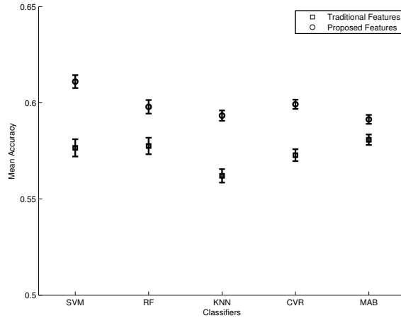
Figure 4: Mean classifier accuracy of two features set (95% CI error bars, note y-axis ranges between 0.5 and 0.65 only)
