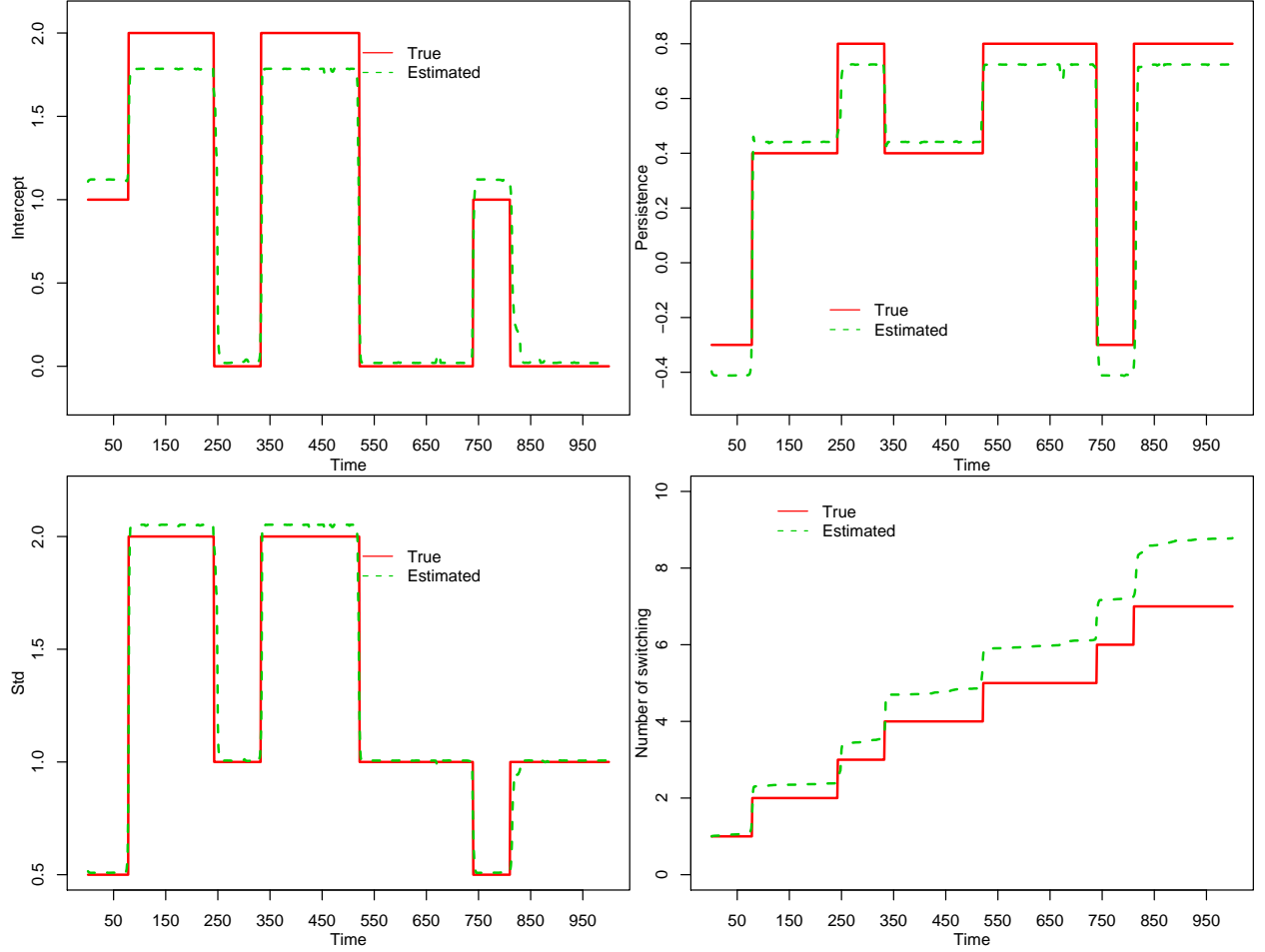
Figure 6: The SDHDP-HMM estimates the data in figure 5. Each state has Gaussian AR(2) dynamics: y_t = \phi_{s_t0} + \phi_{s_t1}y_{t-1} + \phi_{s_t2}y_{t-2} + \sigma_{s_t}\varepsilon_t . The solid lines are the true values and the dashed lines are the posterior means of those values estimated by the SDHDP-HMM. The top-left panel plots the intercepts \phi_{s_t0} ; the top-right panel plots the persistence parameters \phi_{s_t1} + \phi_{s_t2} ; the bottom-left plots the conditional standard deviations \sigma_{s_t} and the bottom-right plots the cumulative number of regime switching.
