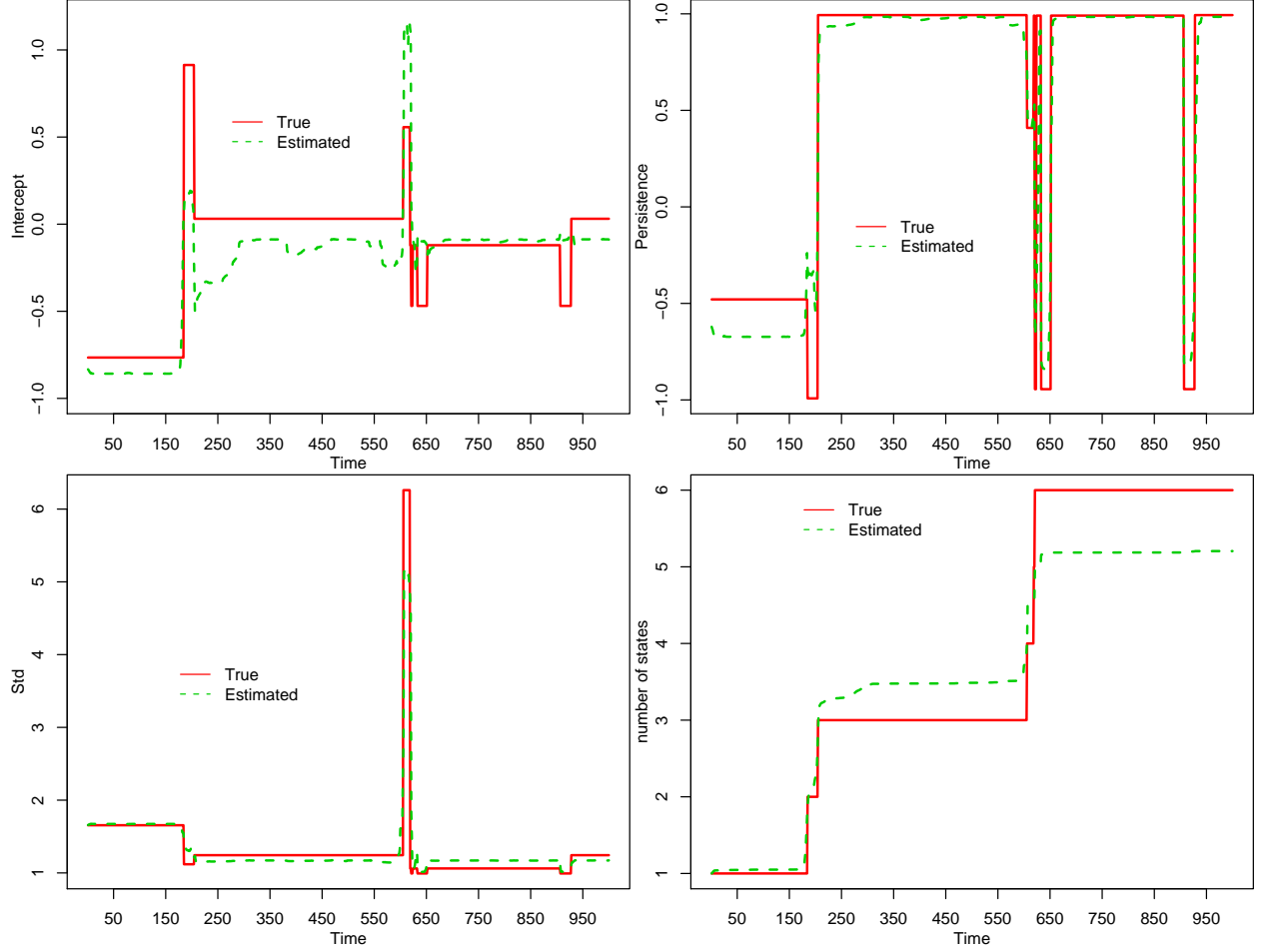
Figure 4: The SDHDP-HMM estimates the data in figure 3. Each state has Gaussian AR(2) dynamics: y_t = \phi_{s_t0} + \phi_{s_t1}y_{t-1} + \phi_{s_t2}y_{t-2} + \sigma_{s_t}\varepsilon_t . The solid lines are the true values and the dashed lines are the posterior means of those values estimated by the SDHDP-HMM. The top-left panel plots the intercepts \phi_{s_t0} ; the top-right panel plots the persistence parameters \phi_{s_t1} + \phi_{s_t2} ; the bottom-left plots the conditional standard deviations \sigma_{s_t} and the bottom-right plots the cumulative number of the active states (active state means it has been visited at least once).
