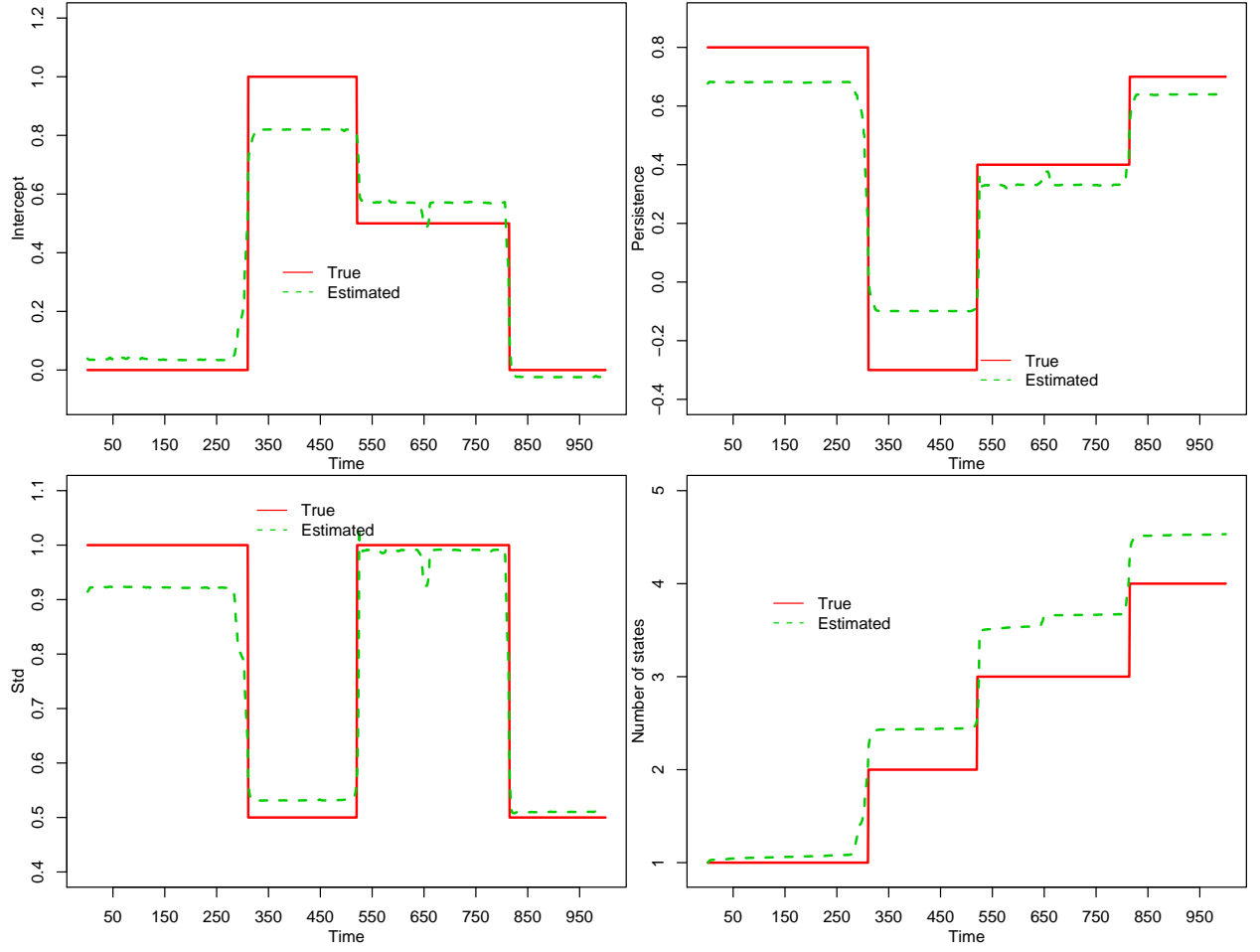
Figure 9: The SDHDP-HMM estimates the data in figure 8. Each state has Gaussian AR(2) dynamics: y_t = \phi_{s_t0} + \phi_{s_t1}y_{t-1} + \phi_{s_t2}y_{t-2} + \sigma_{s_t}\varepsilon_t . The solid lines are the true values and the dashed lines are the posterior means of those values estimated by the SDHDP-HMM. The top-left panel plots the intercepts \phi_{s_t0} ; the top-right panel plots the persistence parameters \phi_{s_t1} + \phi_{s_t2} ; the bottom-left plots the conditional standard deviations \sigma_{s_t} and the bottom-right plots the cumulative number of states.
