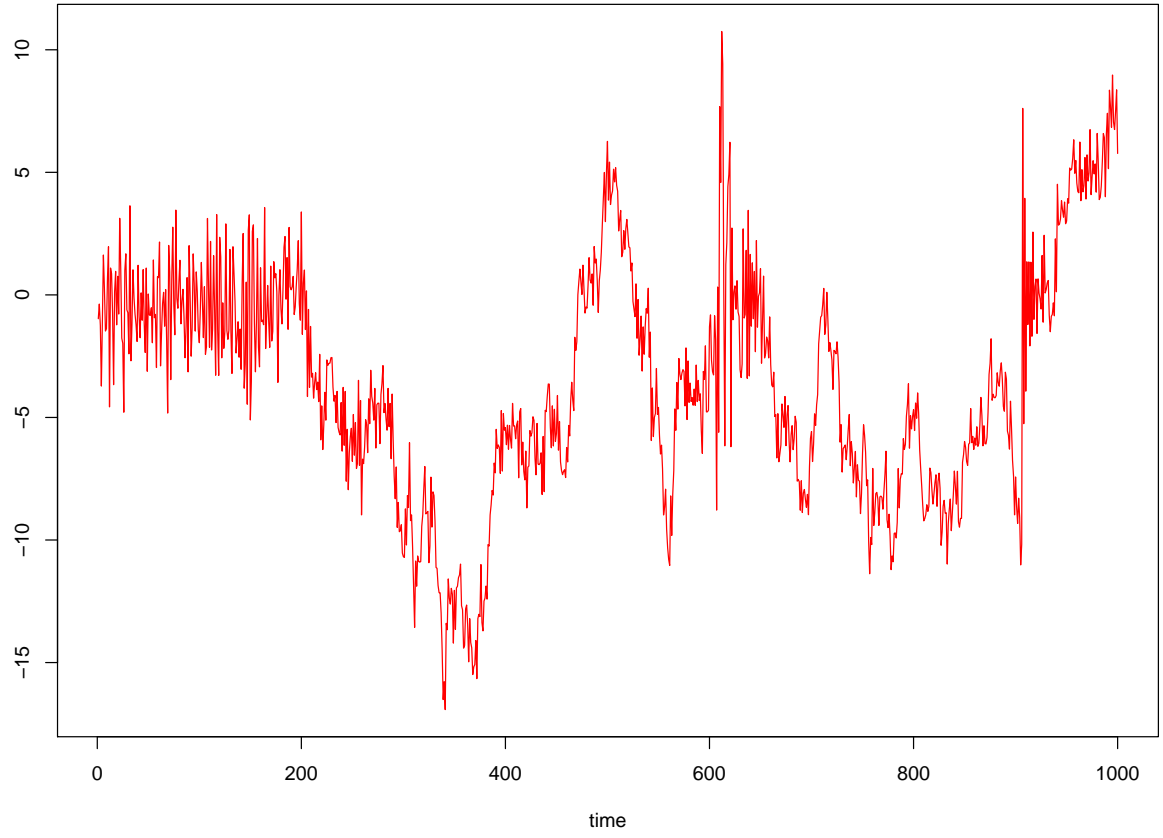
Figure 3: Data simulated by a SDHDP-HMM. Each state has Gaussian AR(2) dynamics: y_t = \phi_{s_t0} + \phi_{s_t1}y_{t-1} + \phi_{s_t2}y_{t-2} + \sigma_{s_t}\varepsilon_t .
