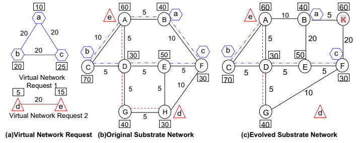
Fig. 1: Virtual Network Request, Original Substrate Network and Evolved Substrate Network
